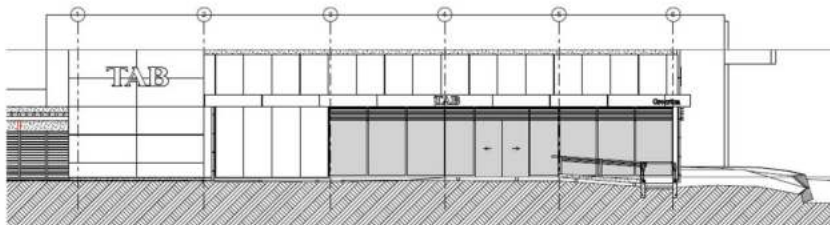
02 South West Elevation Scale 1:100
